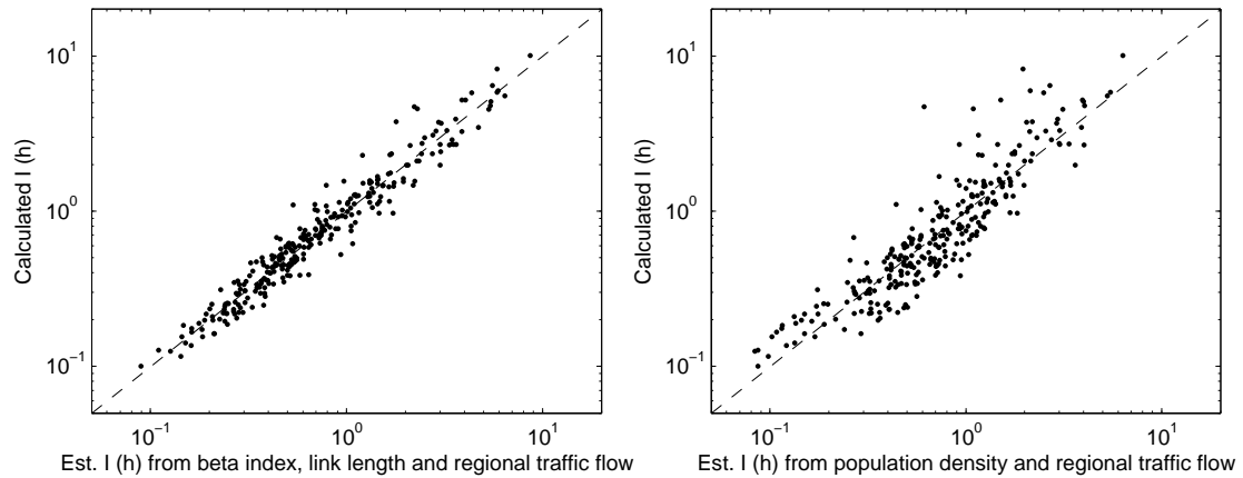
Figure 5: Calculated importance (h) against estimated importance (h) for every municipality. Left: estimate based on beta index, average link length and average regional traffic flow (adj. R^2 = 0.95 ). Right: estimate based on population density and average regional traffic flow (adj. R^2 = 0.81 ). 30 minutes closure, logarithmic scales.
