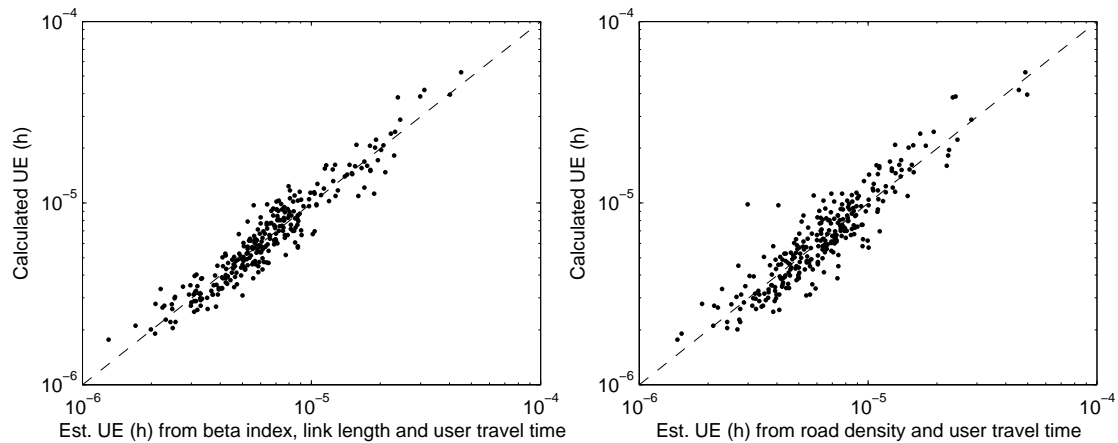
Figure 4: Calculated user exposure (h) against estimated user exposure (h) for every municipality. Left: estimate based on beta index, average link length and average user travel time (adj. R^2 = 0.90 ). Right: estimate based on road density and average user travel time (adj. R^2 = 0.84 ). 30 minutes closure, logarithmic scales.
